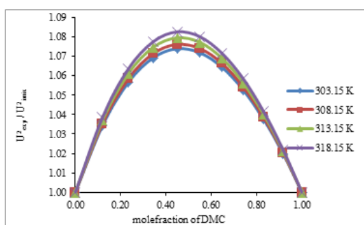
Fig. 1. Variation of U^2_{exp}/U^2_{mix} with mole fraction of DMC in o-cresol
